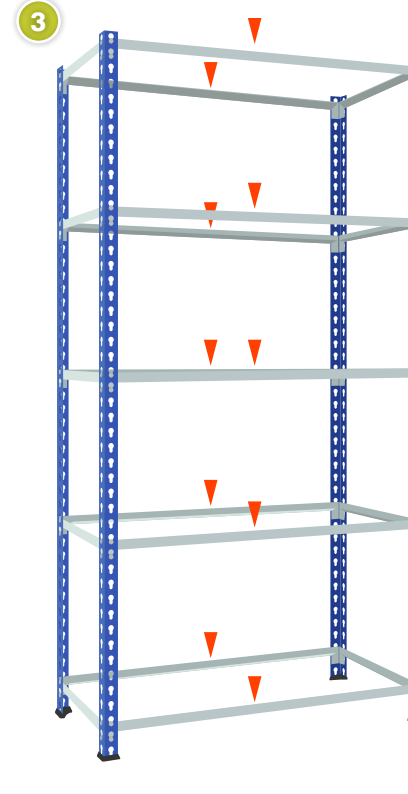
Attach front and back beams to the frames at the same level as the side beams and secure with a rubber mallet.
