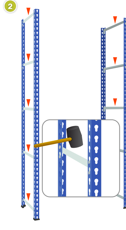
Attach side beams to the uprights at desired heights and secure with a rubber mallet.
